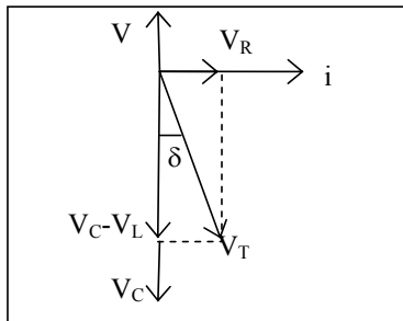
Figure 2: Phasor diagram of capacitor equivalent circuit
